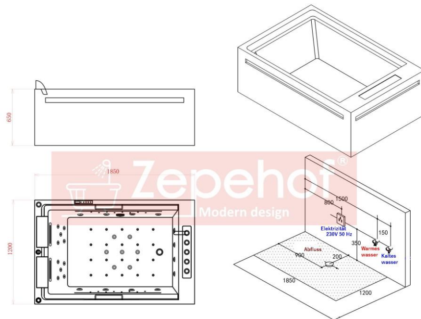
EB-D873 1850*1200*650
